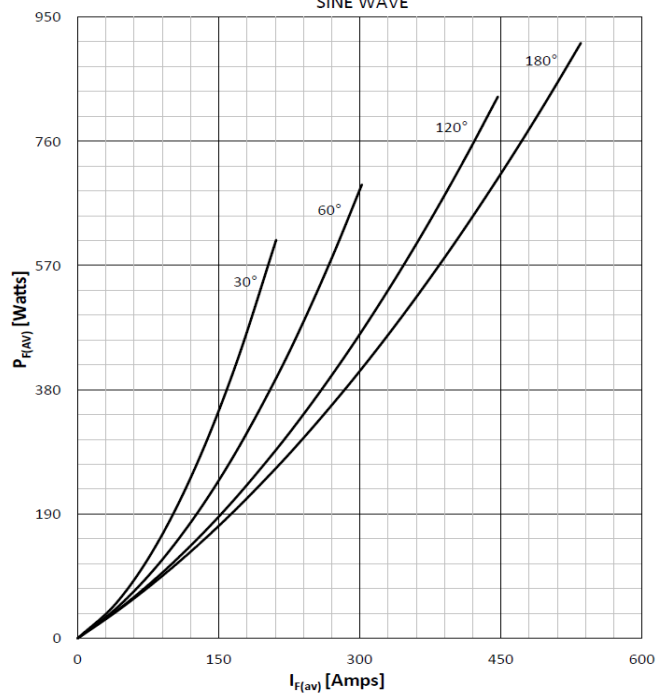
DISSIPATION CHARACTERISTICS
