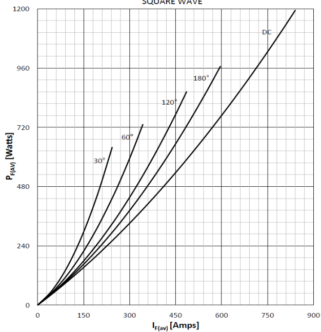
DISSIPATION CHARACTERISTICS
